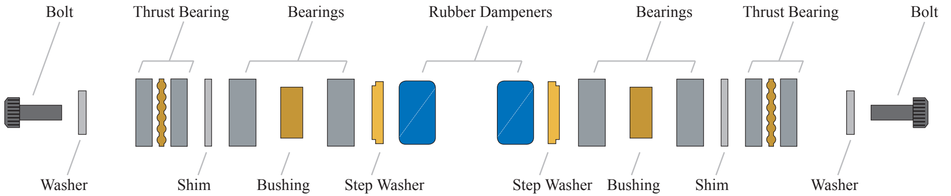
Exploded View
