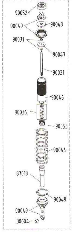
NO. 90056 REAR SHOCK COMPLETE SET
